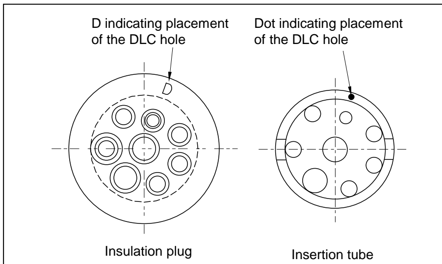
Fig. 3 Placement of DLC hole in insertion tube.
