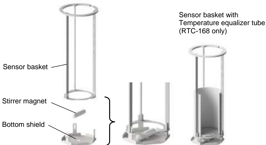
Fig. 4c Sensor basket, stirrer magnet and bottom shield RTC-168
