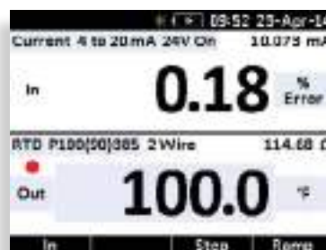
Online % calculation, fast and responsive reading, for calibration and adjustment tasks.
